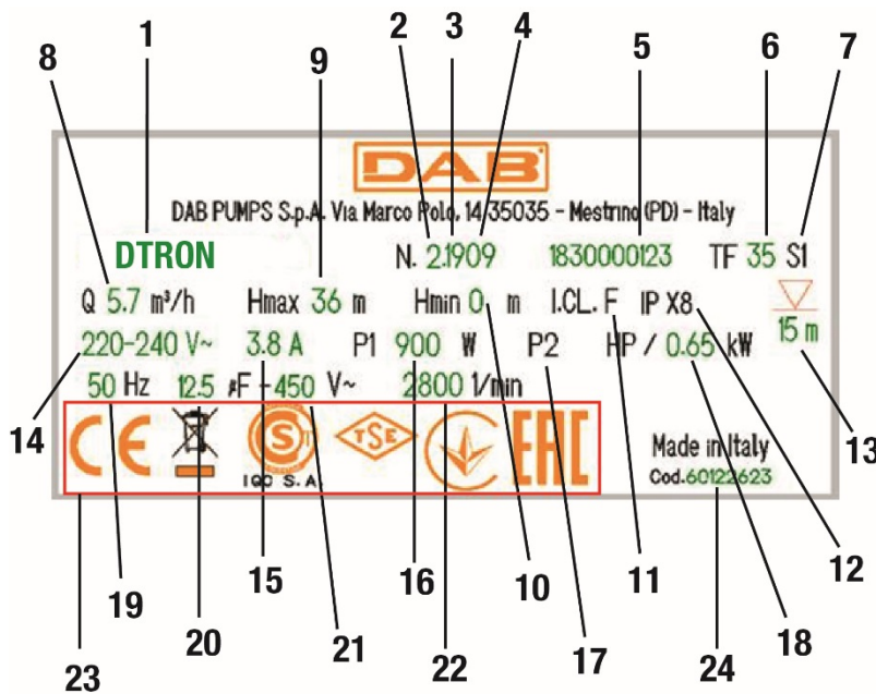
Fig.4 Data plate
